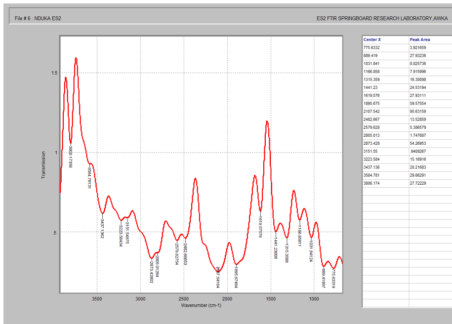
Fig. 9. FTIR of Microplastics from Wetheral, Owerri, Upstream, Otammiri River Sediments
