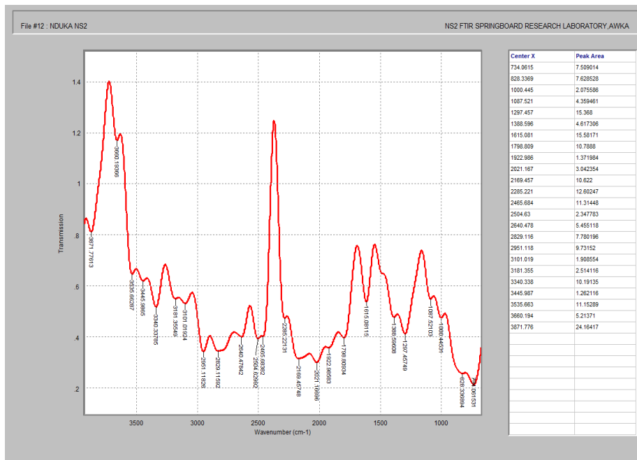
Fig. 8. FTIR of Microplastics from Nekede, Otammiri River Sediments
