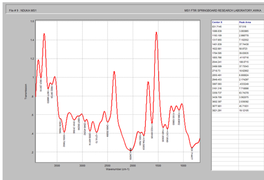
Fig. 2. FTIR of Microplastics from Ekwuato, Downstream of Otammiri River Surfaces
