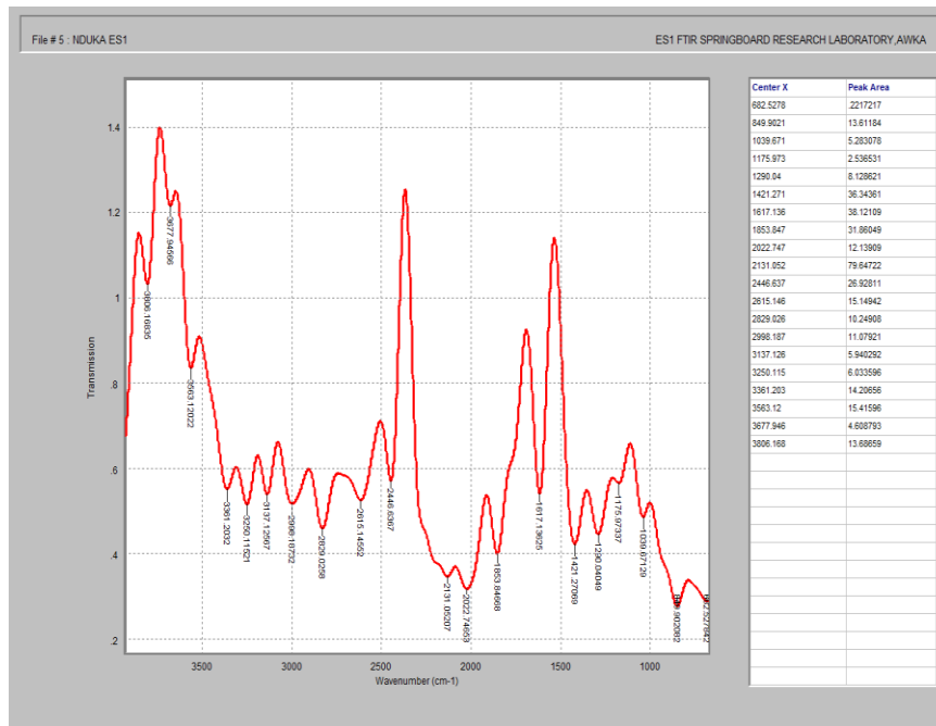
Fig. 5. FTIR of Microplastics from Wetheral, Owerri, Upstream, Otammiri River
