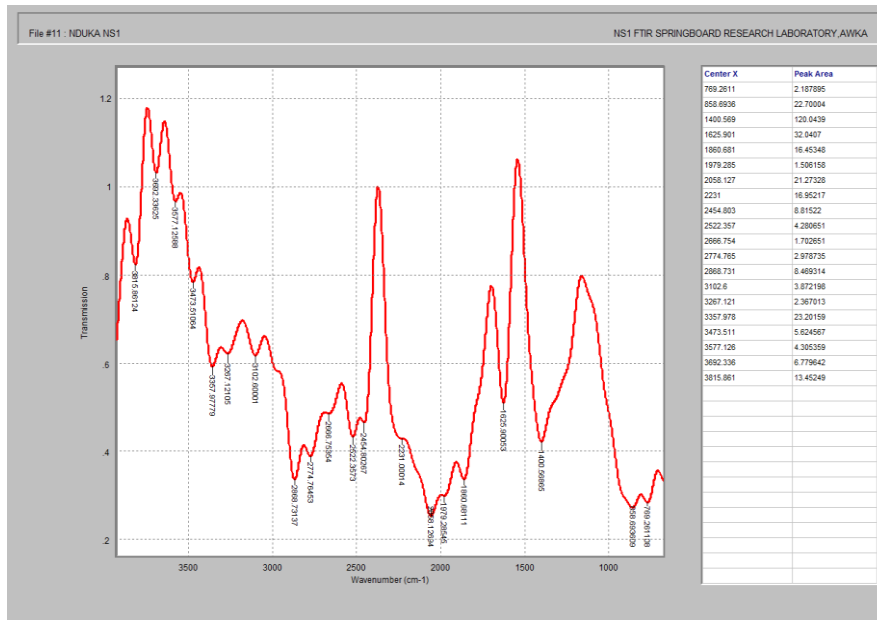
Fig. 4. FTIR of Microplastics from Nekede 460106, Otammiri River Surfaces
