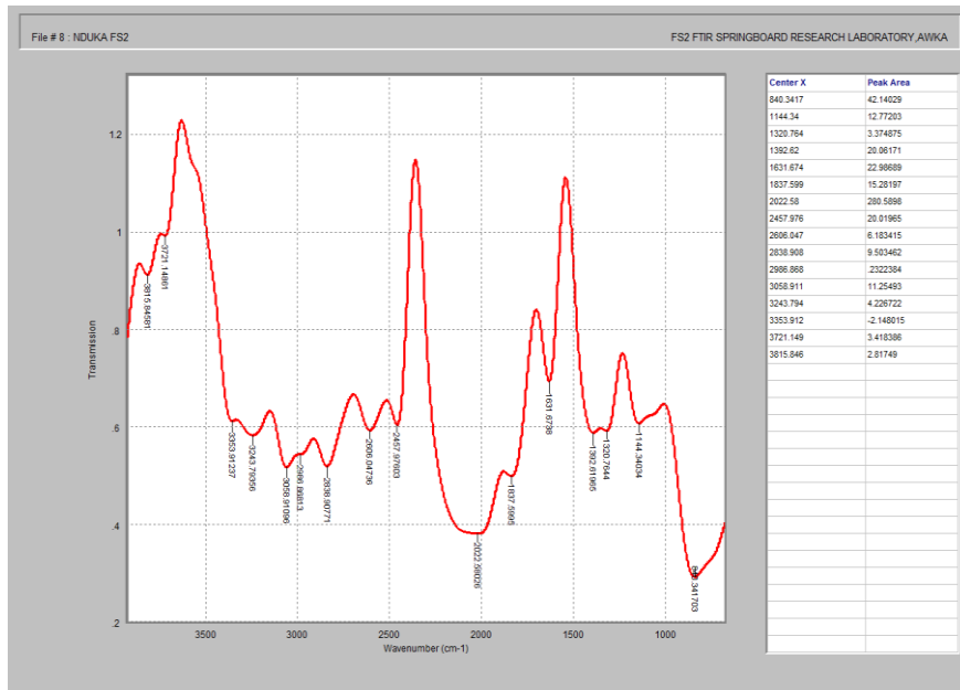
Fig. 7. FTIR of Microplastics from Ihiagwa, Otammiri River Sediments
